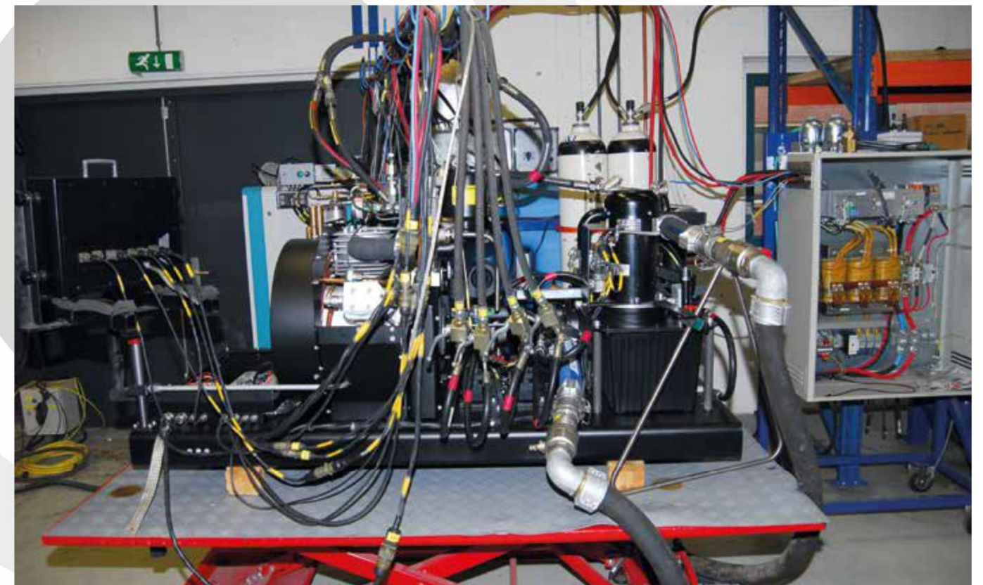
Arrangement of an IFEX® firefighting unit in the testing laboratory
